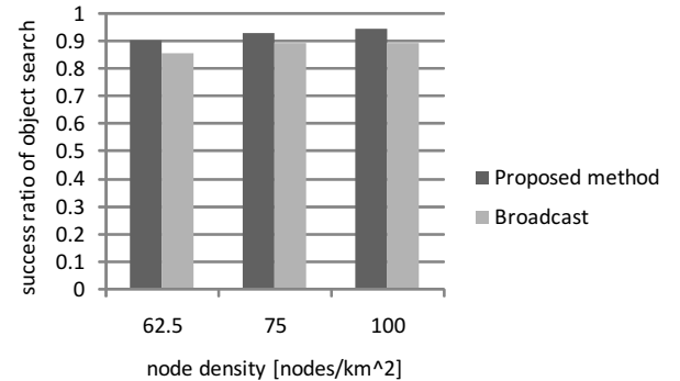
Fig. 12 Success ratio of object search when changing node density
